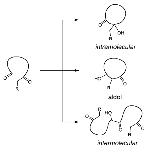
Figure 1. Competing reaction pathways.
