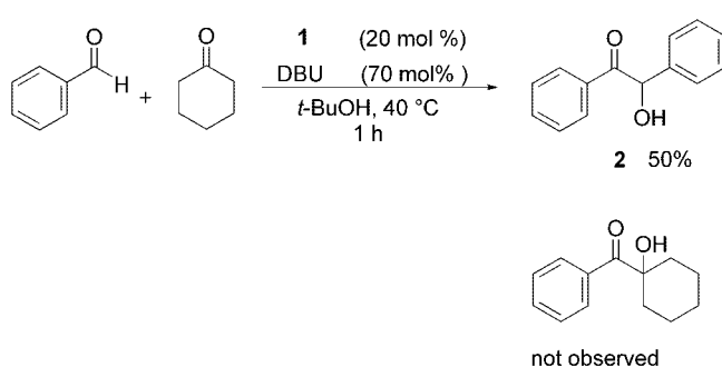
Scheme 3. Intermolecular benzoin-forming reaction.
