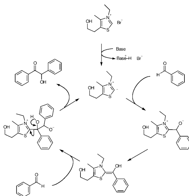
Scheme 1. Proposed mechanism of thiazolium ylide-catalyzed reaction.
